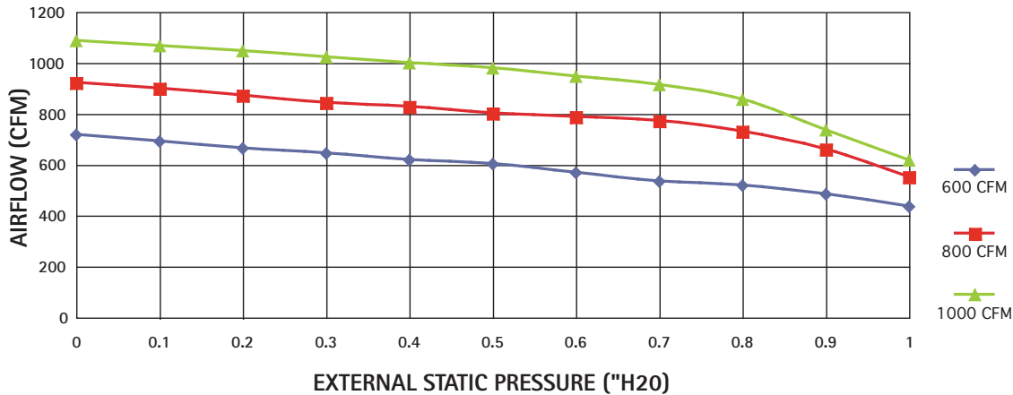
RXAH46 AIRFLOW vs EXTERNAL STATIC
